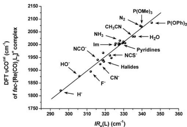
Figure 8. Plot of DFT-calculated symmetric C≡O stretching frequencies ( A_1 mode) of octahedral fac - [\text{Re}(\text{CO})_3\text{L}_3]^n complexes (DFT \nu_{\text{COcat}} , y axis, \text{cm}^{-1} ) versus the corresponding IR_p(\text{L}) value ( x axis, \text{cm}^{-1} ). The plot shows the linear relationship between DFT \nu_{\text{COcat}} and IR_p(\text{L}) of 26 complexes. The IR_p(\text{CN}^-) value of 317.2 \text{ cm}^{-1} was derived from [\text{AsPh}_4][\text{Re}(\text{CO})_3(\text{CN})_3] (Supporting Information). A 5 \text{ cm}^{-1} correction was applied to the IR_p(\text{P(OPh)}_3) value according to Table 1, footnote h .
