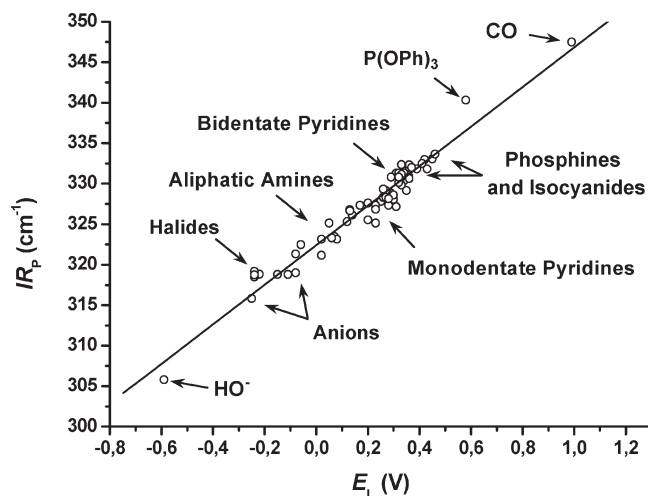
Figure 3. Plot of IR_{\text{P}}(\text{L}) parameters ( y axis, \text{cm}^{-1} ) versus their corresponding E_{\text{L}} values ( x axis, V).
